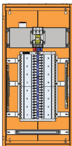
FRONT VIEW WITH DOOR AND ESCUTCHEON REMOVED
